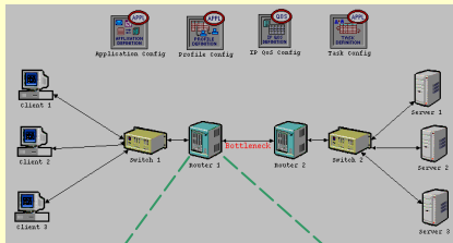
IP network model: packet scheduling is implemented in IP routers 1 and 2.
