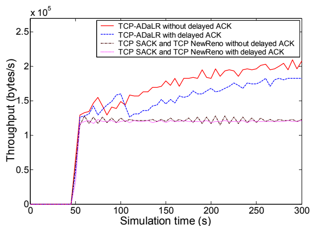
Figure 2. Scenario with an ideal lossless satellite channel. TCP-ADaLR shows up to 63% higher throughput than TCP SACK and TCP NewReno with delayed ACK disabled.
