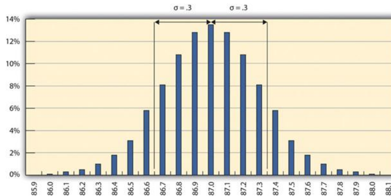
Figure 14.2 One Sigma Range
