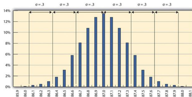
Figure 14.3 The 68-95-99.7 Rule
