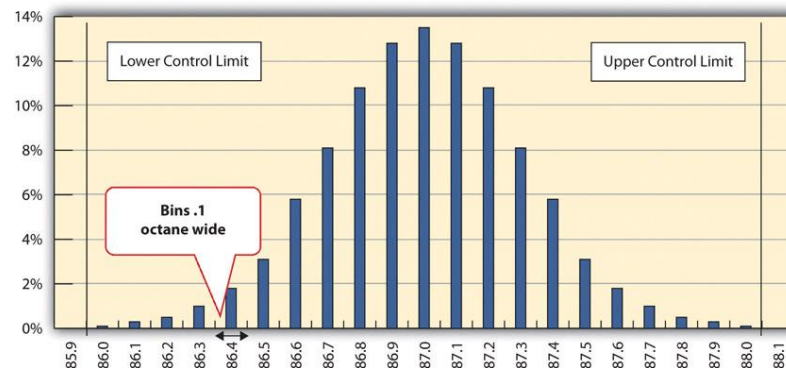
Figure 14.1 Normal Distribution of Measurements
